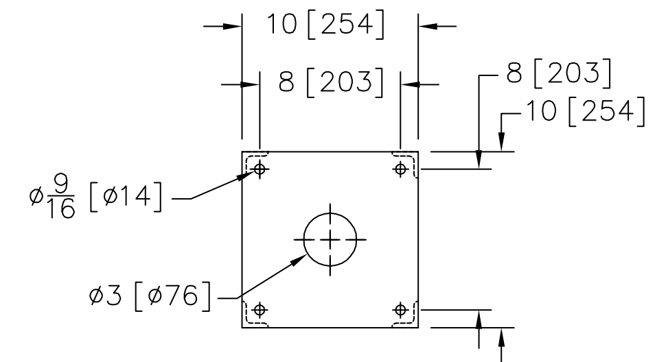
WSB 140R FOOTPRINT
