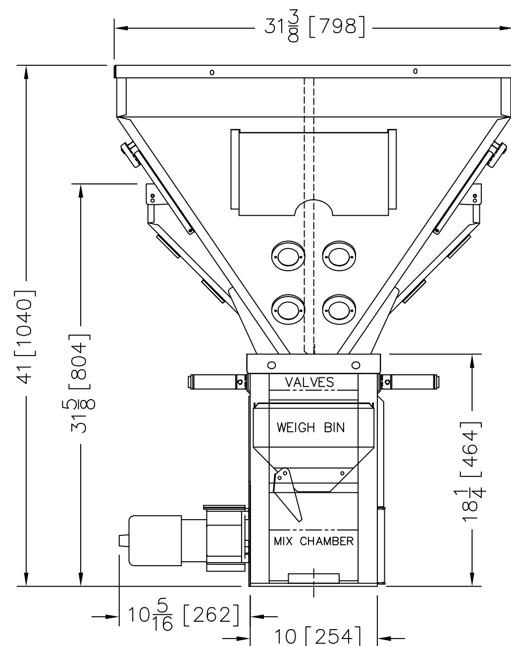
WSB 140R SIDE VIEW
