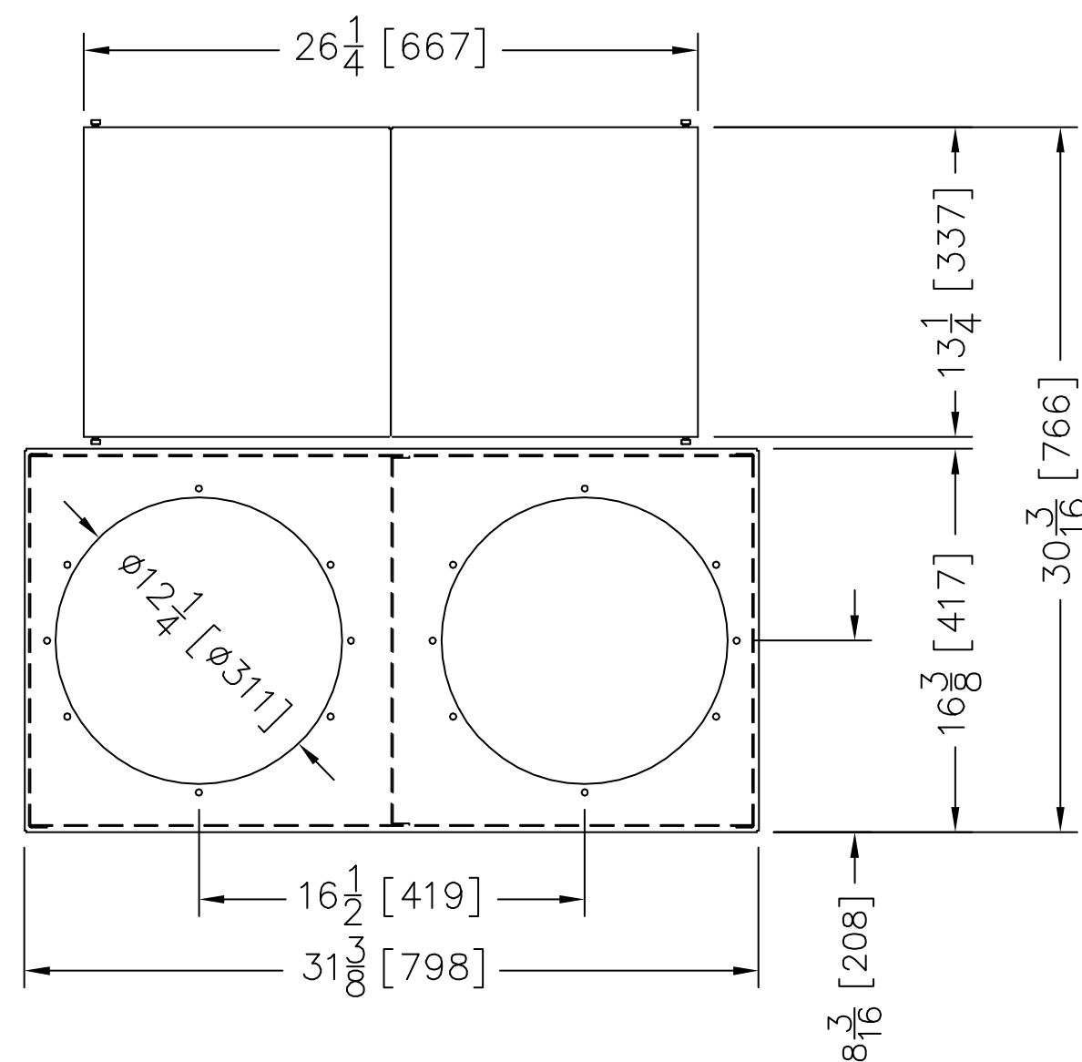
WSB 140R SIDE VIEW
