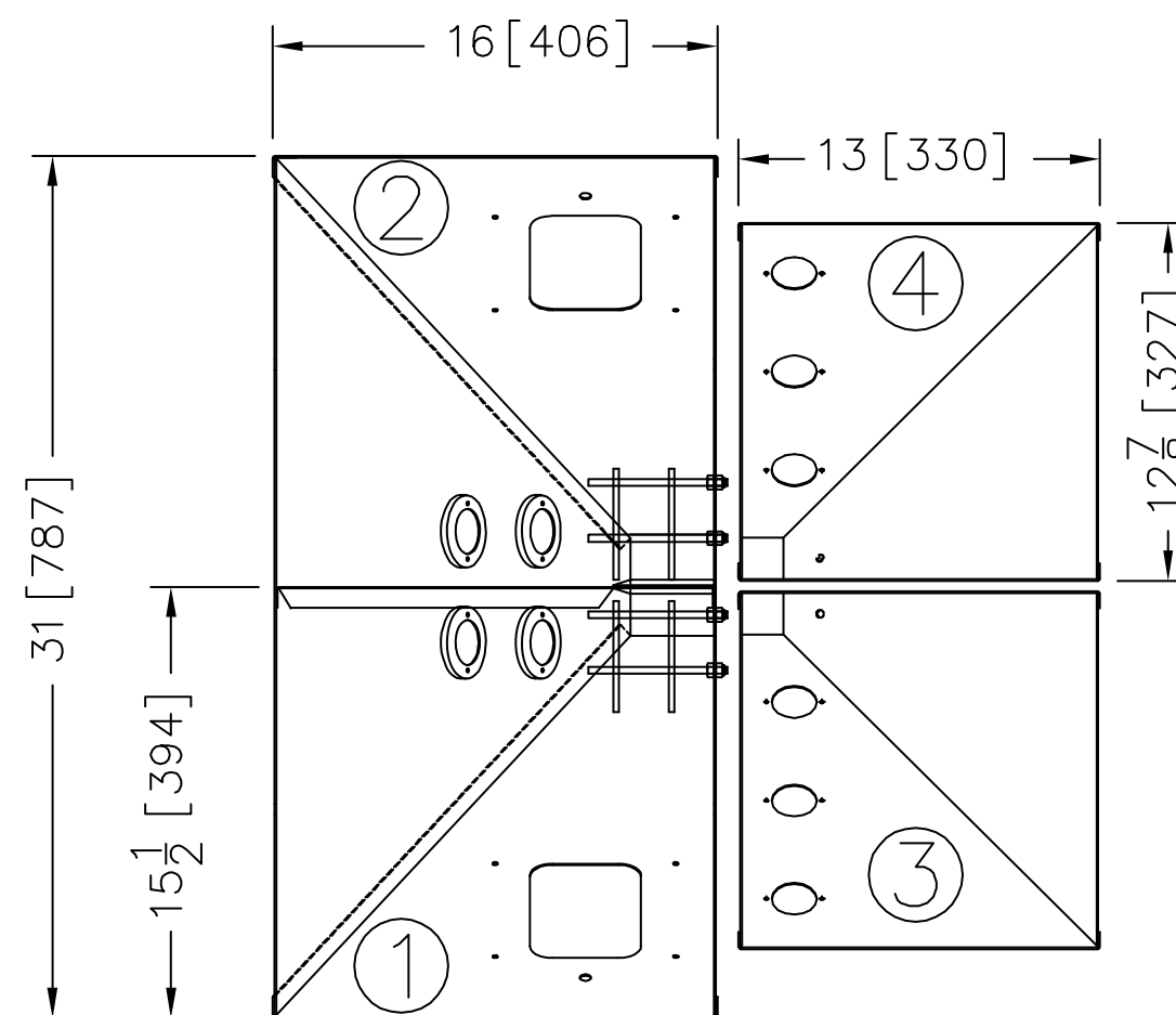
WSB 140R FRONT VIEW
