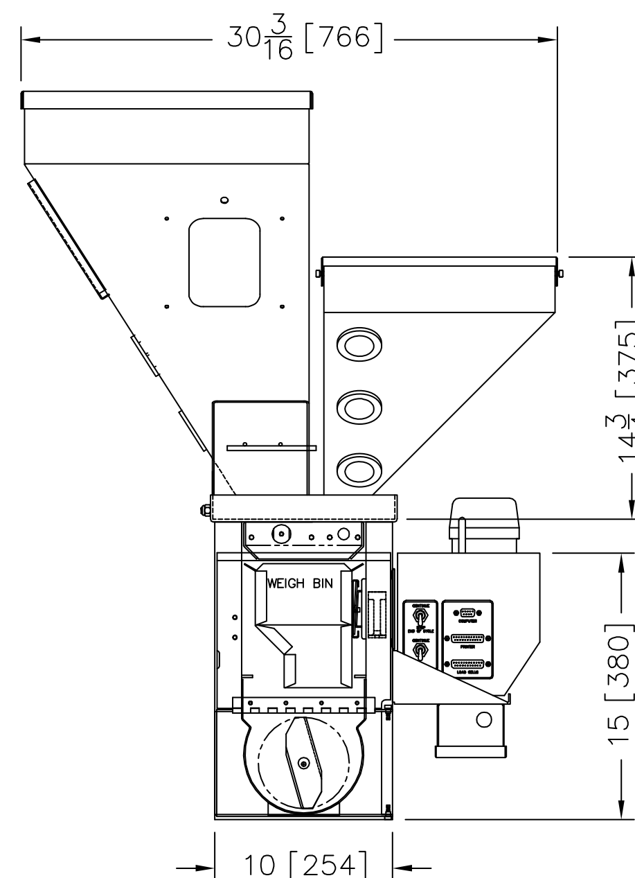
WSB 140R FRONT VIEW
