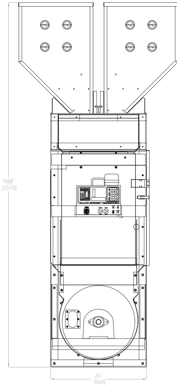
WSB 3060 FRONT VIEW
