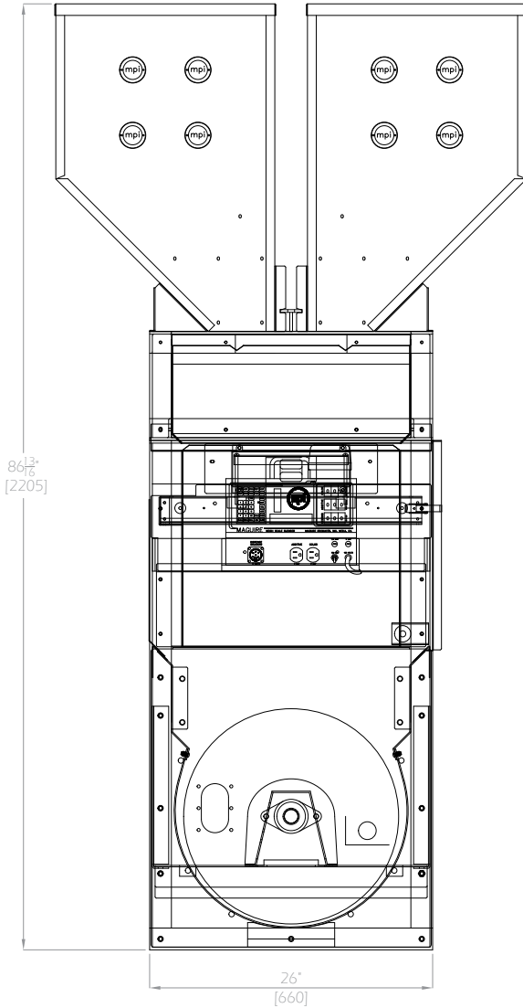
WSB 2460 FRONT VIEW
