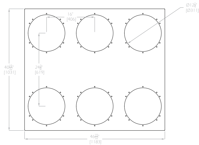
WSB-1860 FRONT VIEW
