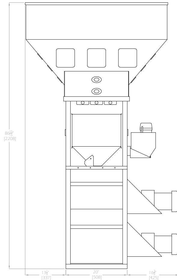
WSB-1860 FRONT VIEW
