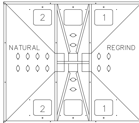
WSB-1820 HOPPER TOP VIEW
