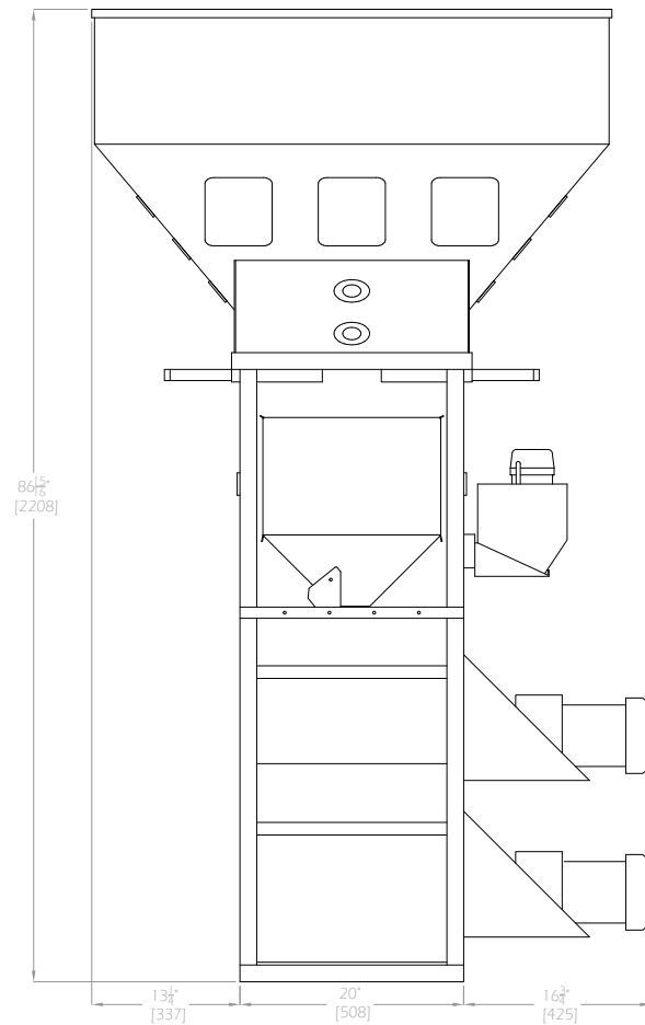
WSB-1820 FRONT VIEW
