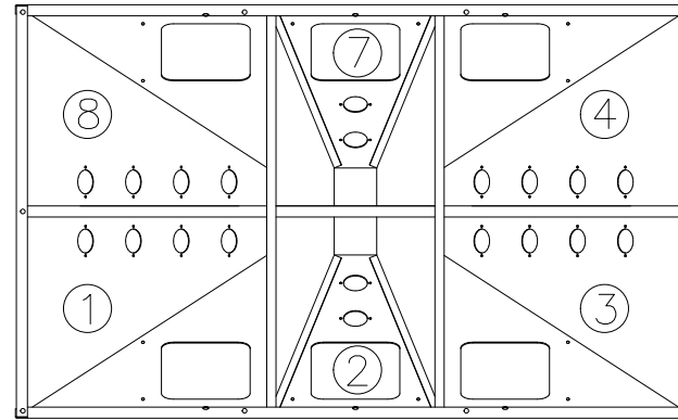
WSB-960 HOPPER TOP VIEW
