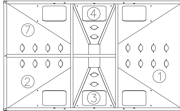
WSB-950 HOPPER TOP VIEW
