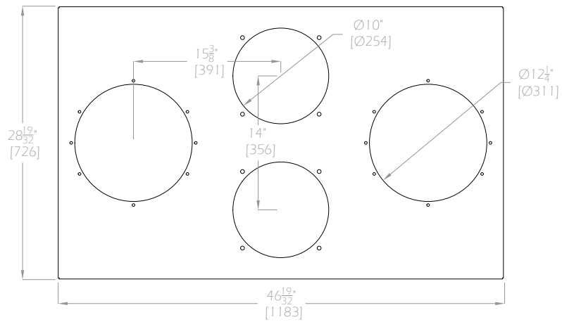
WSB-940 FRONT VIEW
