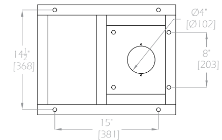
WSB-940 Footprint
