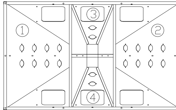
WSB-940 HOPPER TOP VIEW
