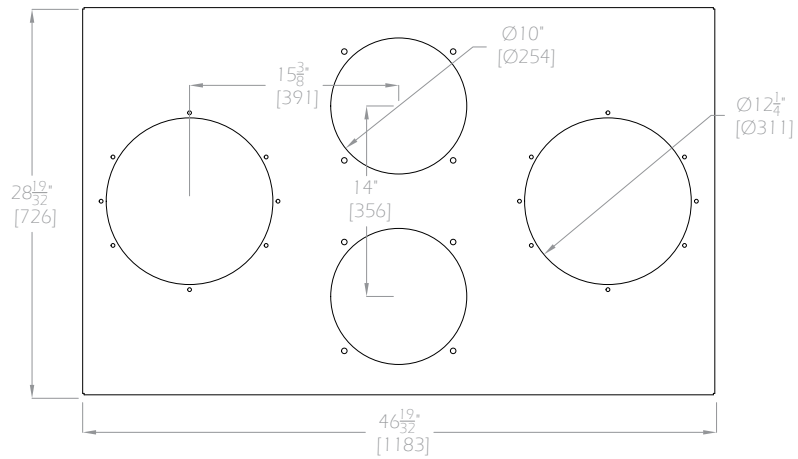
WSB-920 FRONT VIEW
