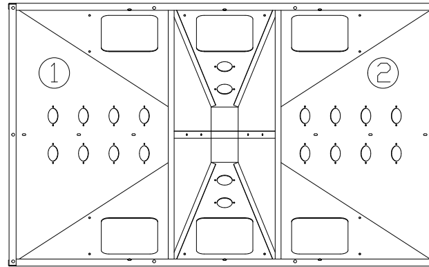
WSB-920 HOPPER TOP VIEW
