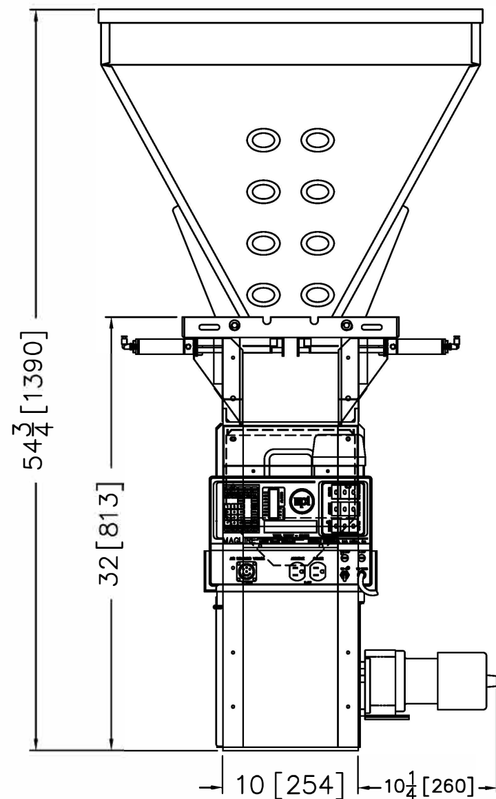
WSB 460 SIDE VIEW
