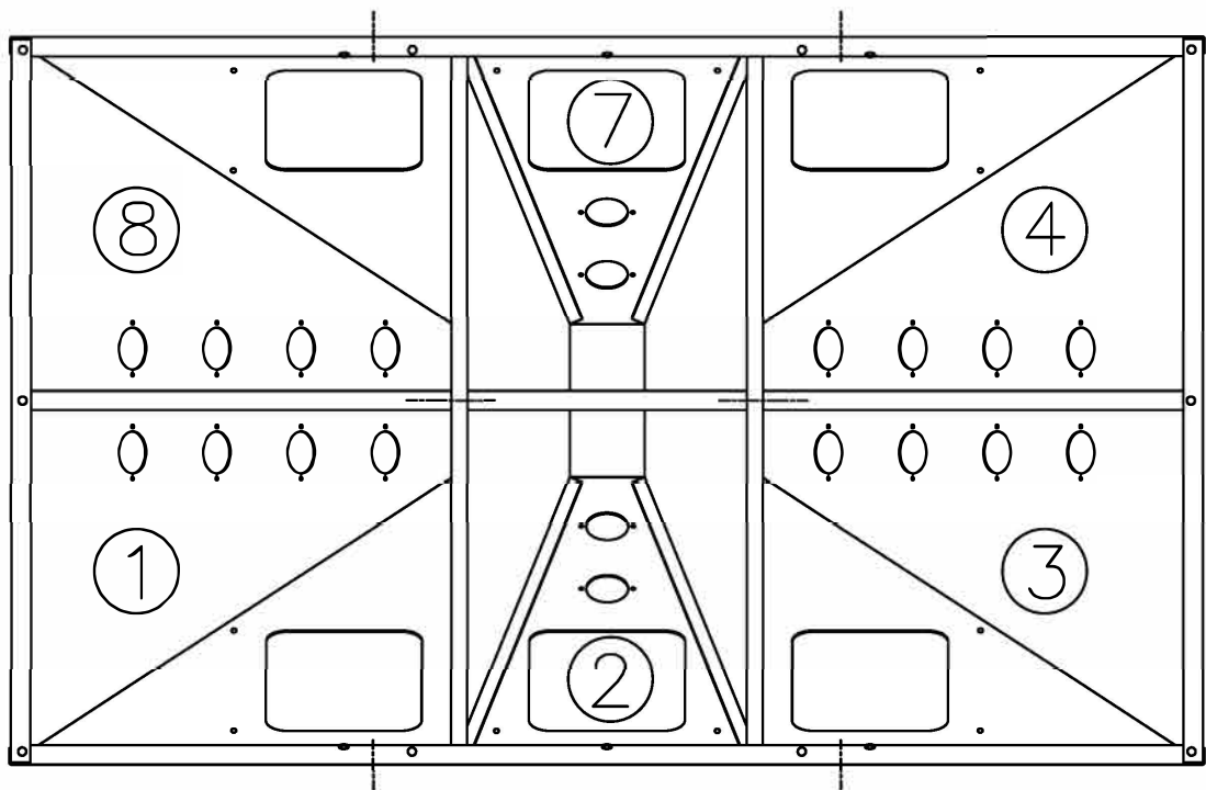
WSB 460 / 960 HOPPER TOP VIEW CONTROLLER SIDE
