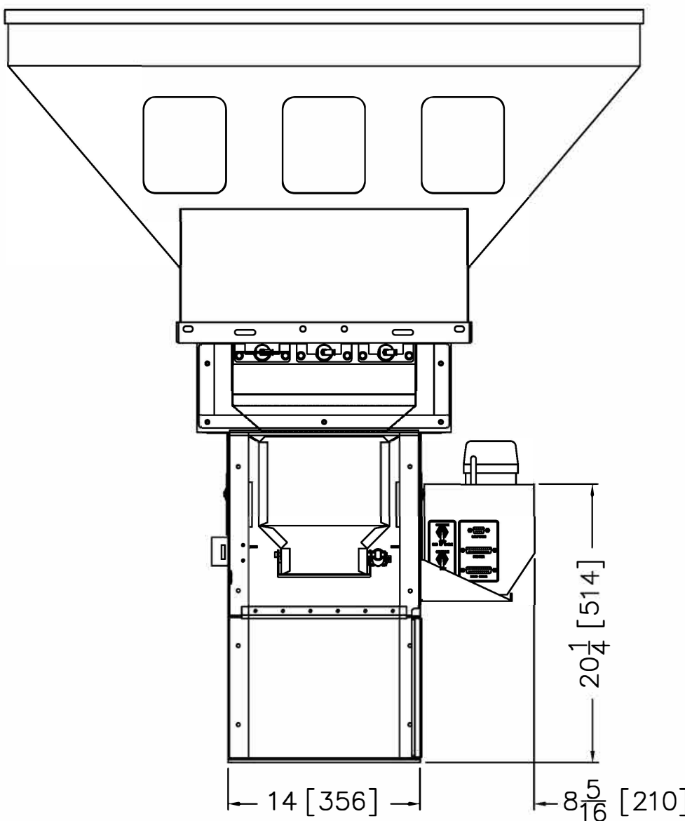
WSB 460 FRONT VIEW
