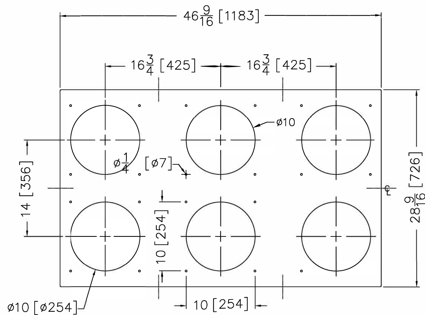
WSB 460 SIDE VIEW
