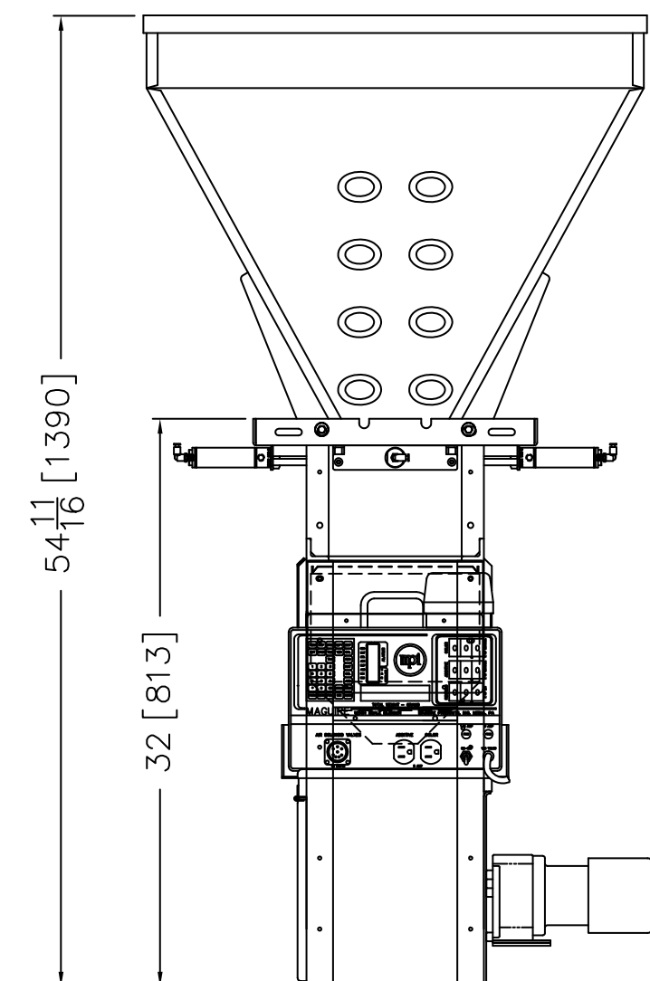
WSB 450 SIDE VIEW
