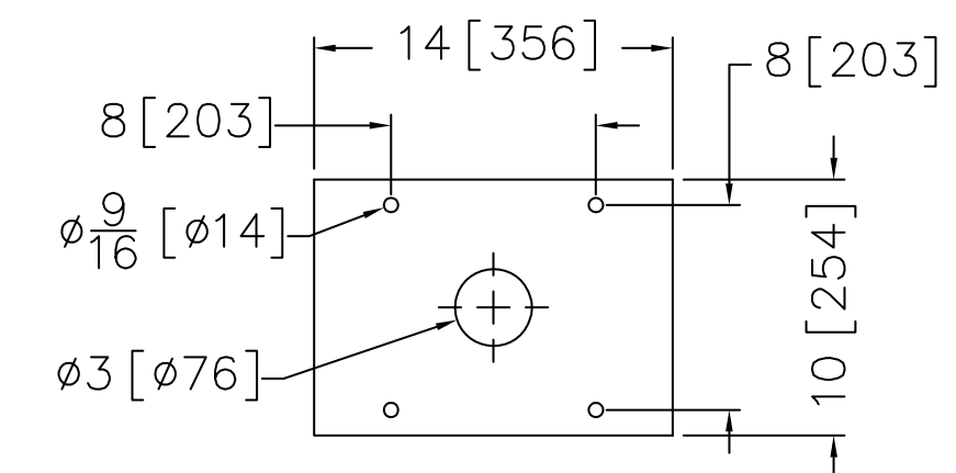
WSB 450 FOOTPRINT
