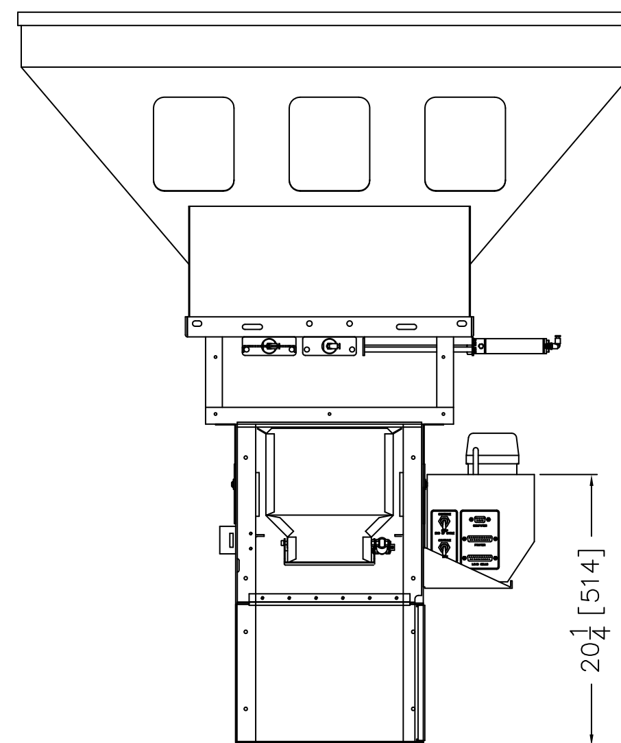
WSB 450 FRONT VIEW
