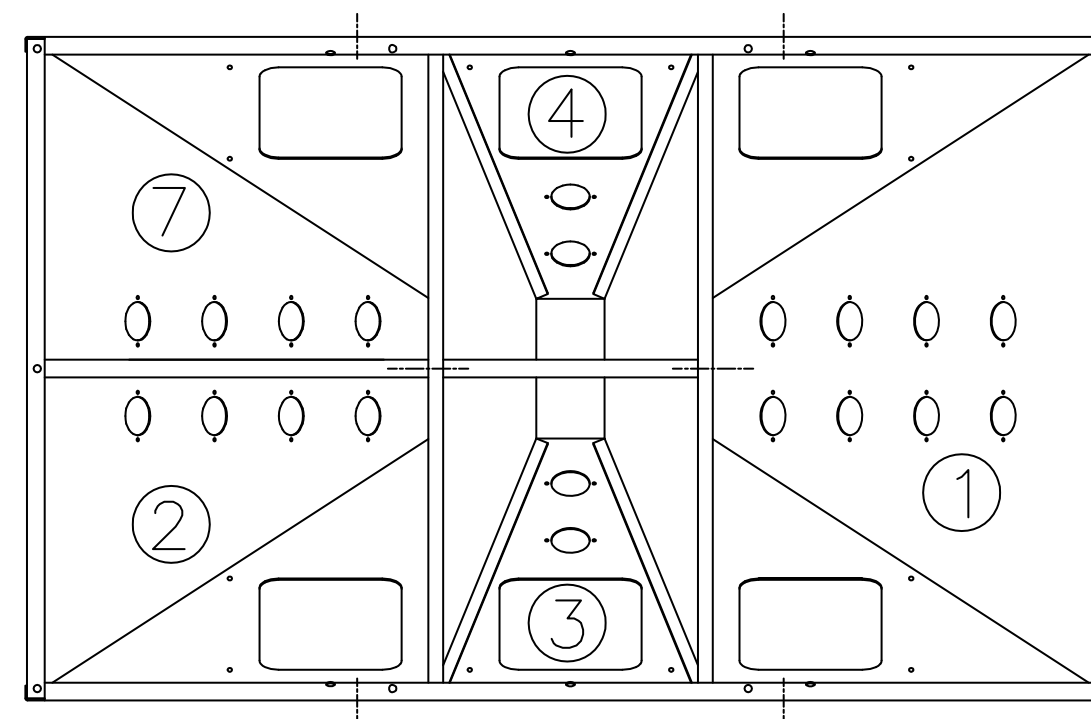
WSB 450 HOPPER TOP VIEW CONTROLLER SIDE
