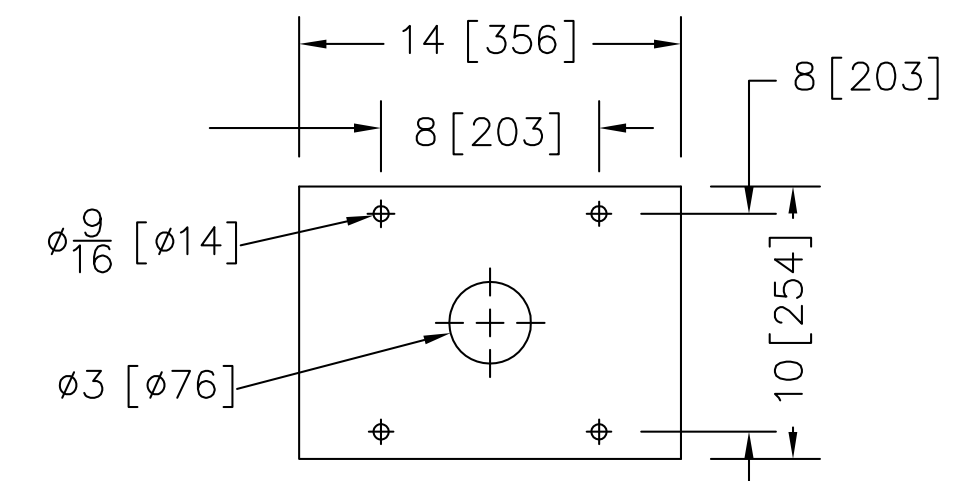
WSB 440 FOOTPRINT
