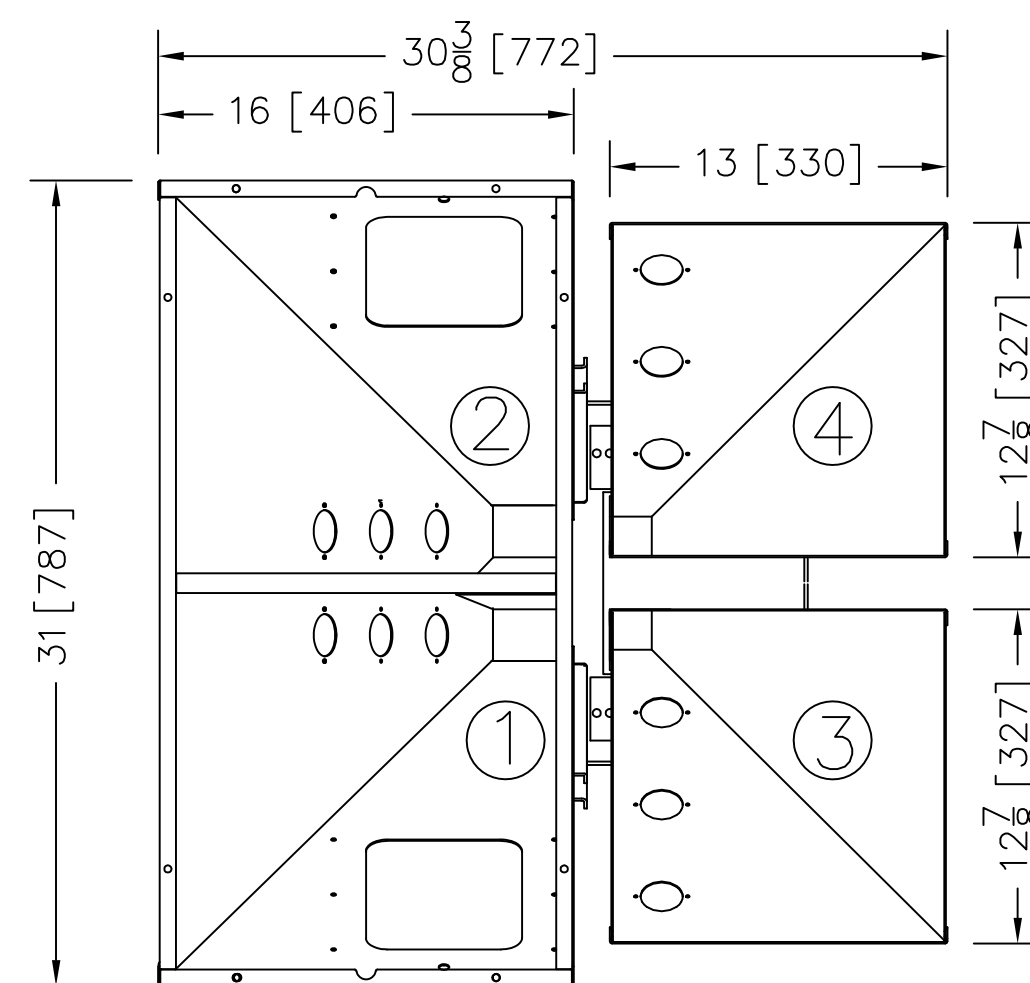
WSB 440 HOPPER TOP VIEW
