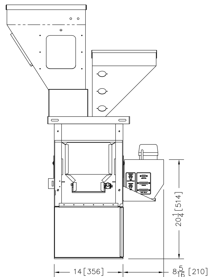
WSB 440 SIDE VIEW
