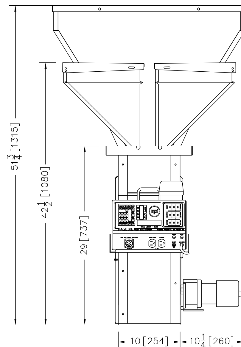
WSB 440 FRONT VIEW
