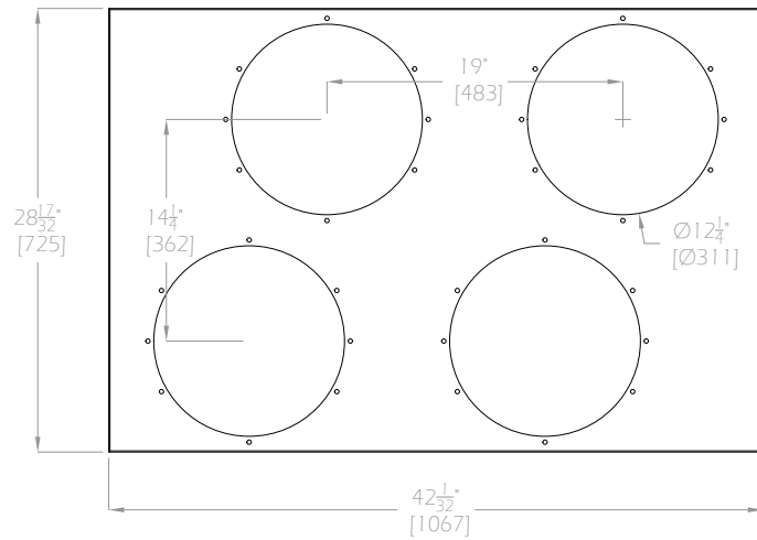
WSB-440 FRONT VIEW
