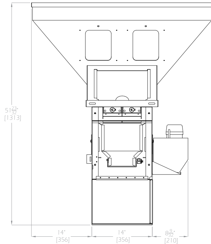
WSB-440 FRONT VIEW
