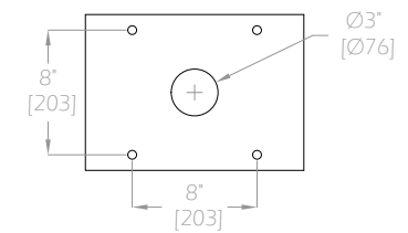
STD WSB Bottom Plate
