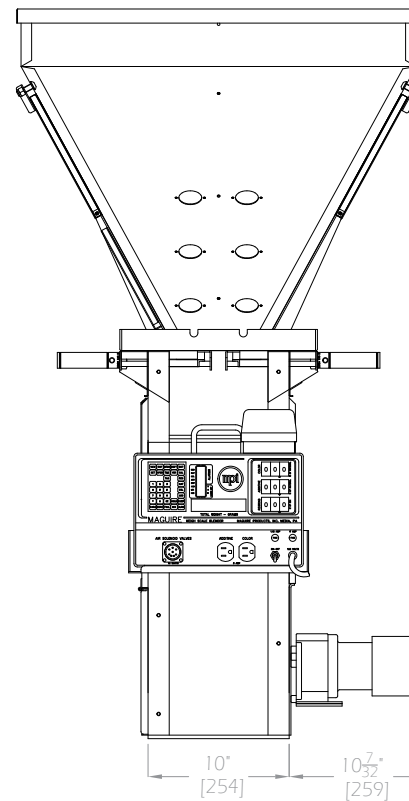
WSB-440 SIDE VIEW
