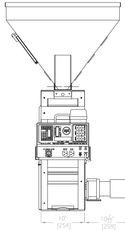
WSB-420 SIDE VIEW
