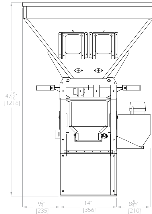
WSB-420 FRONT VIEW
