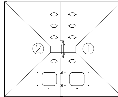
WSB-420 HOPPER TOP VIEW
