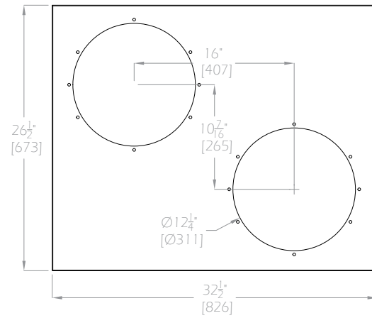
WSB-420 FRONT VIEW
