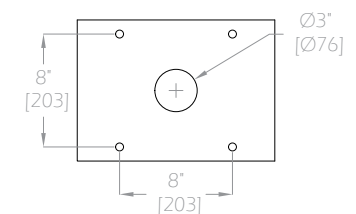
WSB-260 Footprint
