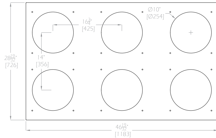
WSB-260 FRONT VIEW
