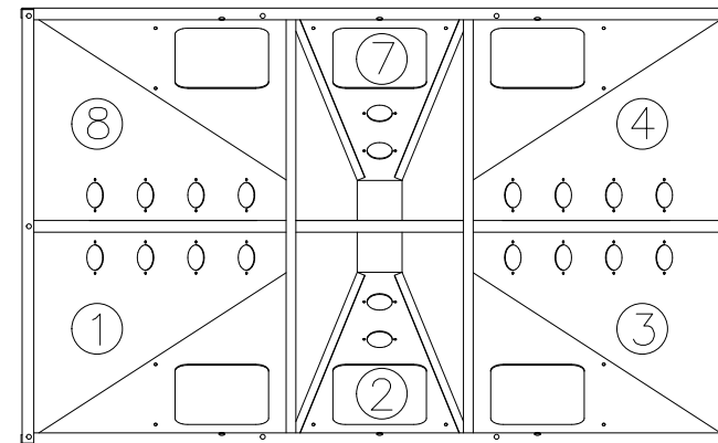
WSB-260 HOPPER TOP VIEW
