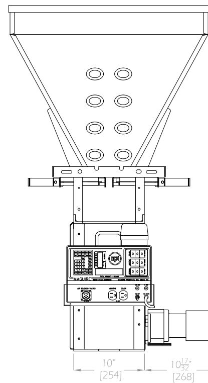
WSB-260 SIDE VIEW
