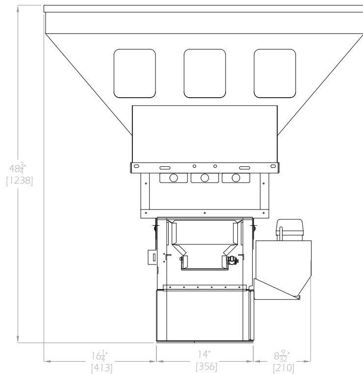
WSB-260 FRONT VIEW
