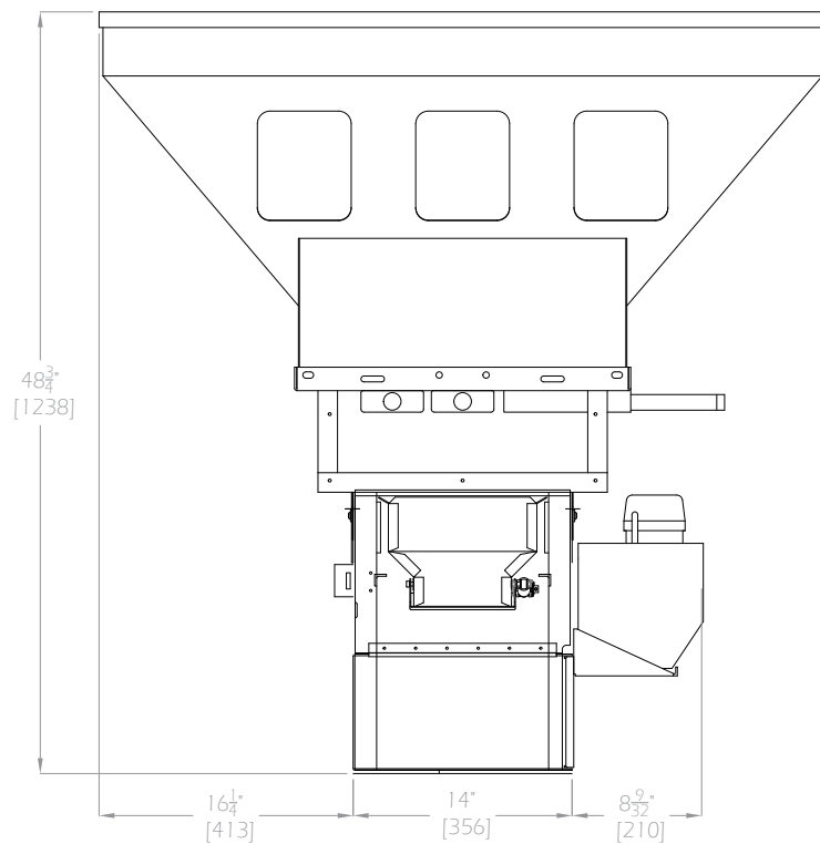
WSB-250 FRONT VIEW
