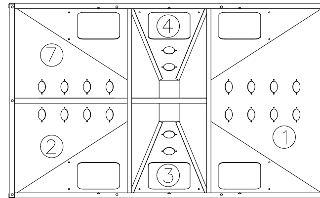
WSB-250 HOPPER TOP VIEW
