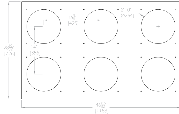
WSB-250 FRONT VIEW
