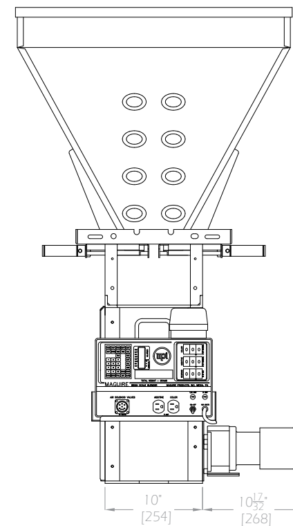
WSB-250 SIDE VIEW
