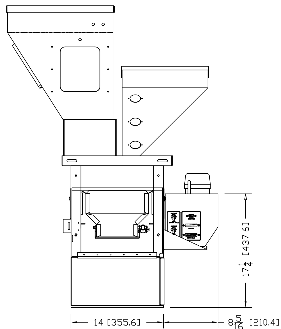
WSB 240 SIDE VIEW
