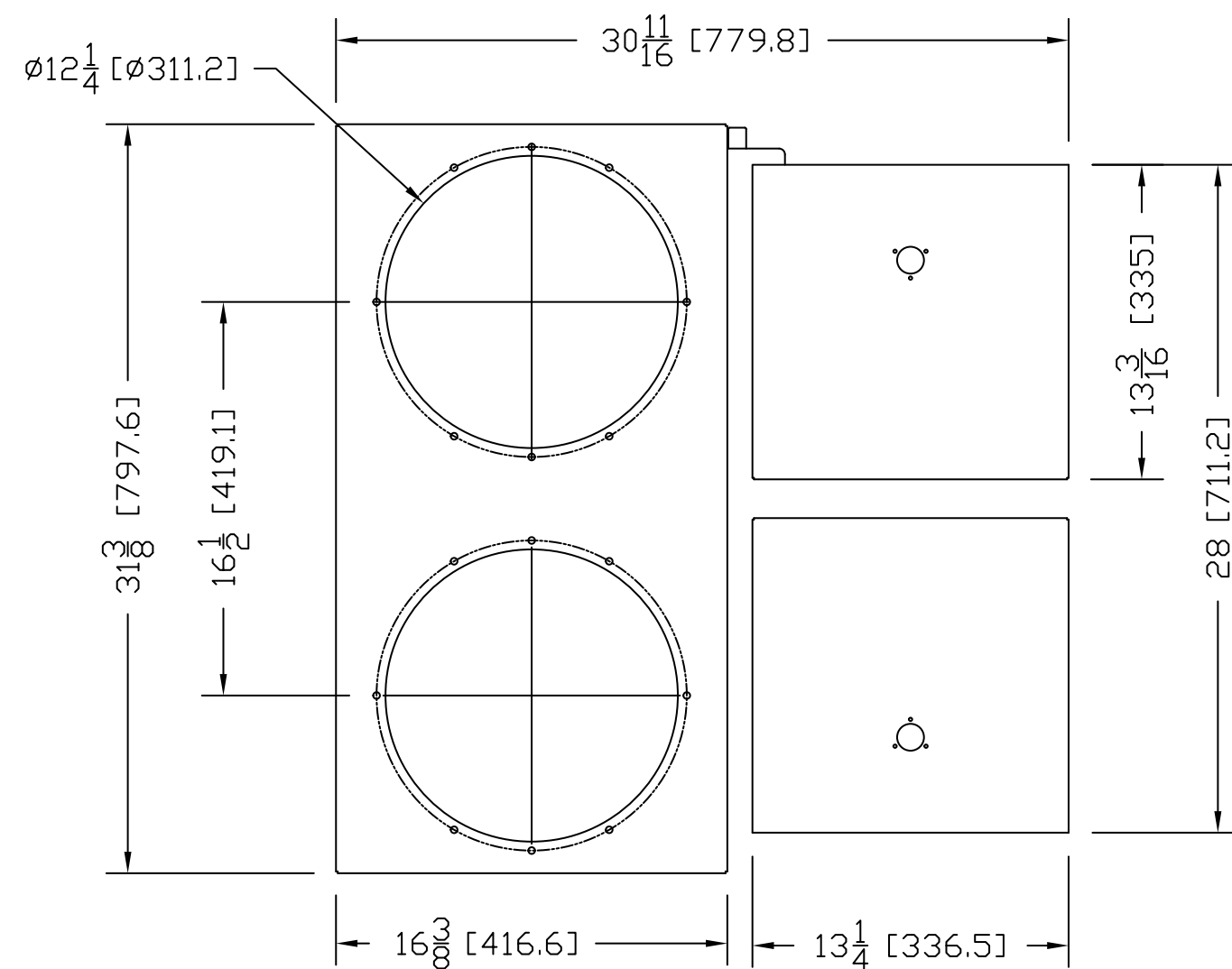
WSB 240 SIDE VIEW
