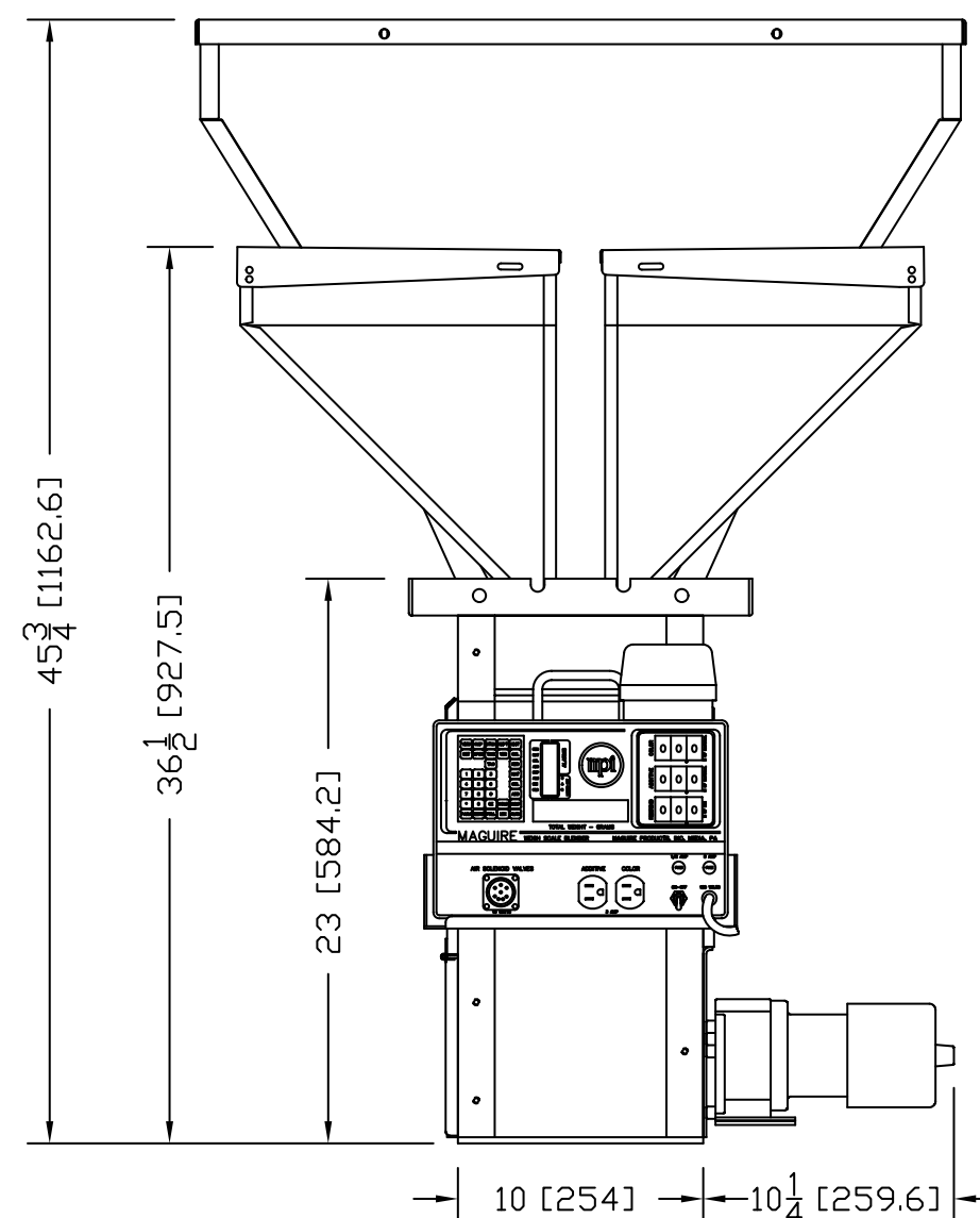
WSB 240 FRONT VIEW
