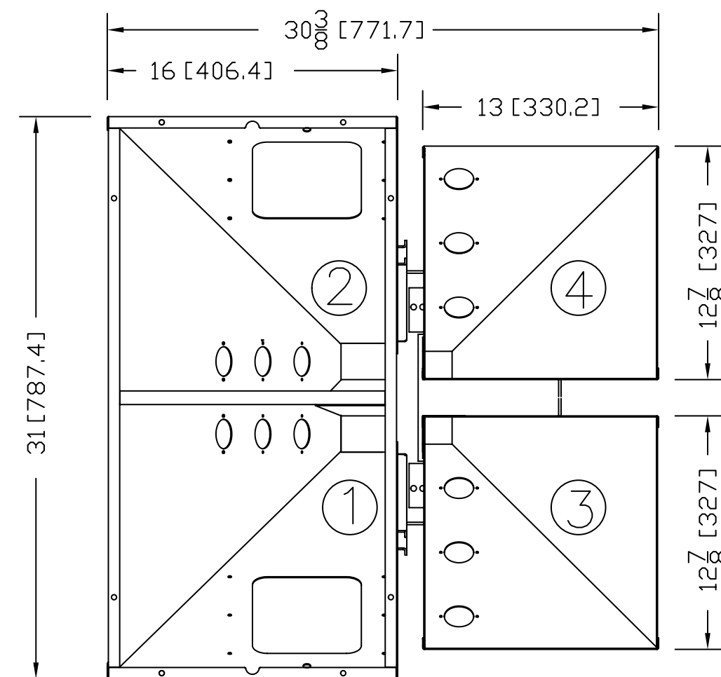
WSB 240 HOPPER TOP VIEW
