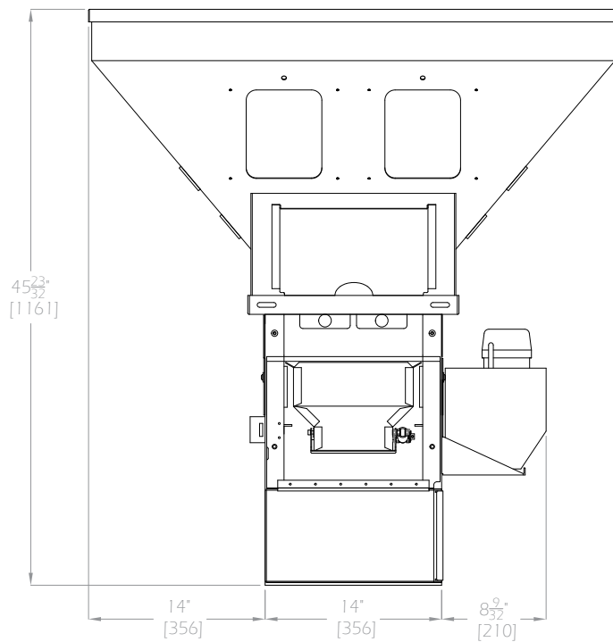
WSB-240 FRONT VIEW
