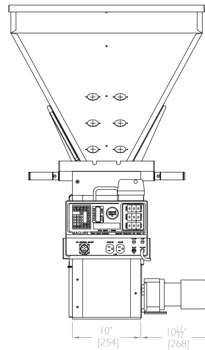
WSB-240 SIDE VIEW
