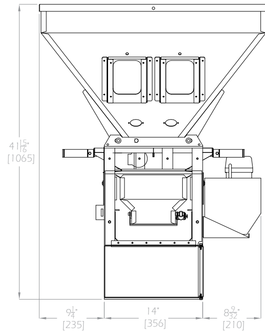
WSB-220 FRONT VIEW
