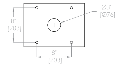
STD WSB Bottom Plate
