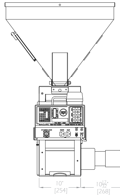
WSB-220 SIDE VIEW
