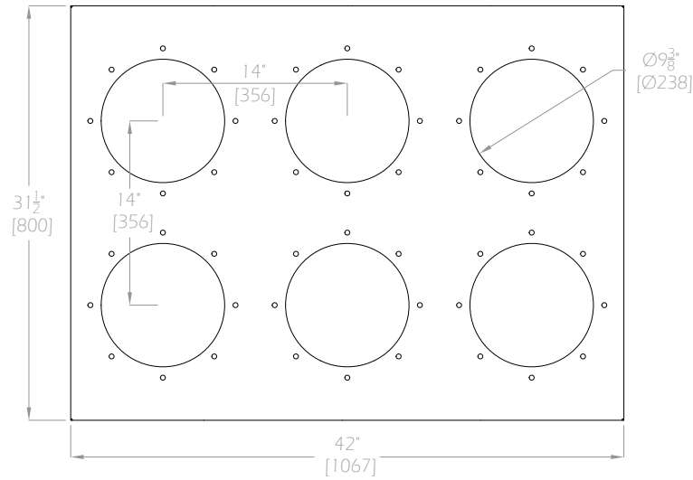
WSB-160 FRONT VIEW
