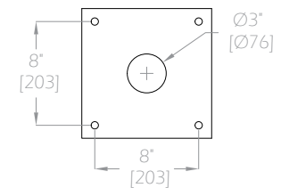
STD WSB Bottom Plate 1/4" [6.4] Steel Plate
