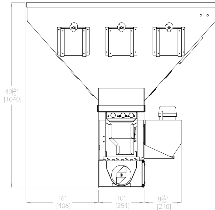
WSB-160 FRONT VIEW
