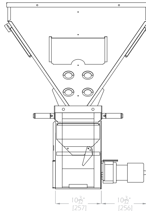
WSB-160 SIDE VIEW
