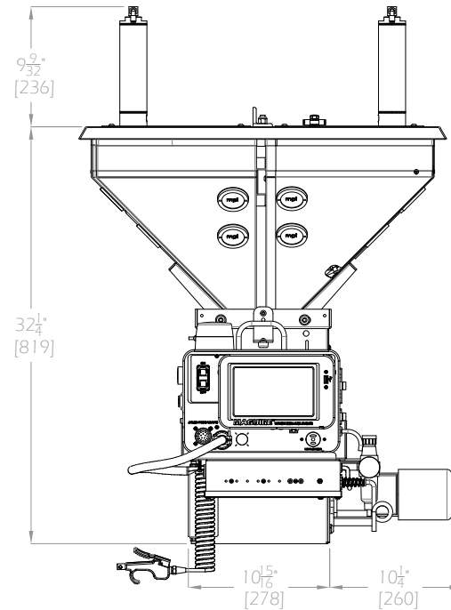
WSB-150MP SIDE VIEW Lid Closed
