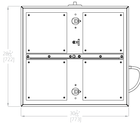
WSB-150MP LID TOP VIEW
