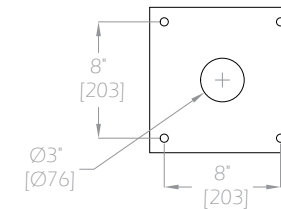
STD WSB Bottom Plate \frac{1}{4}" [6.4] Steel Plate
