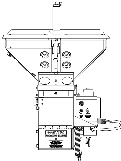
WSB-150MP SIDE VIEW Lid Closed
