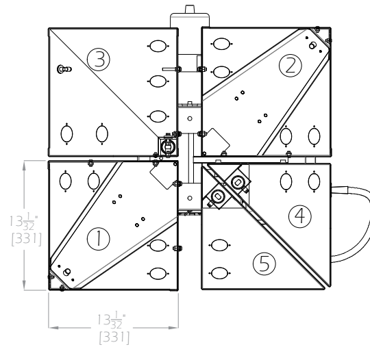
WSB-150MP HOPPER VIEW
