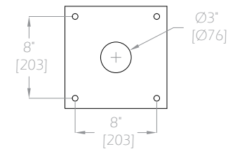
STD WSB Bottom Plate \frac{1}{4}" [6.4] Steel Plate
