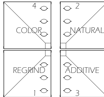
WSB-140MP HOPPER TOP VIEW Mix Motor Side
