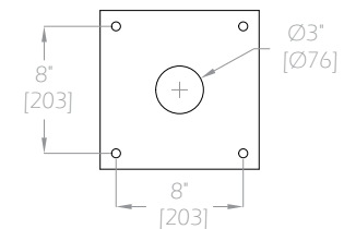
WSB-140MP Footprint
