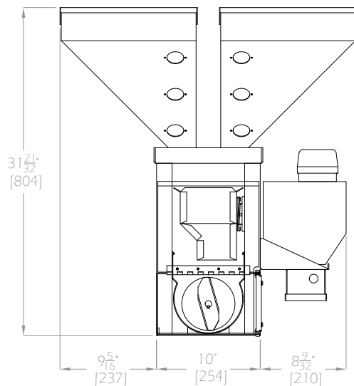
WSB-140MP FRONT VIEW
