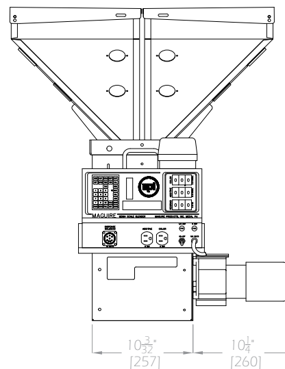
WSB-140MP SIDE VIEW
