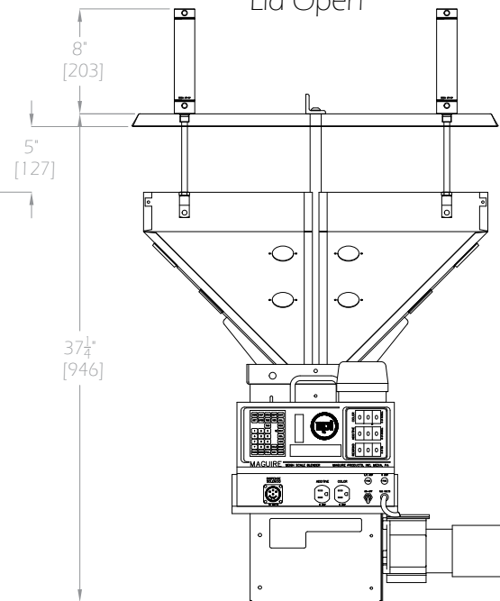
WSB-140MP SIDE VIEW Lid Open
