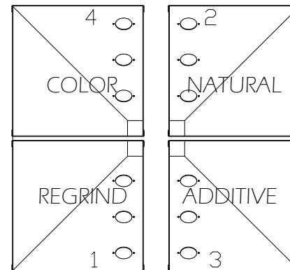
WSB-140MP HOPPER TOP VIEW
