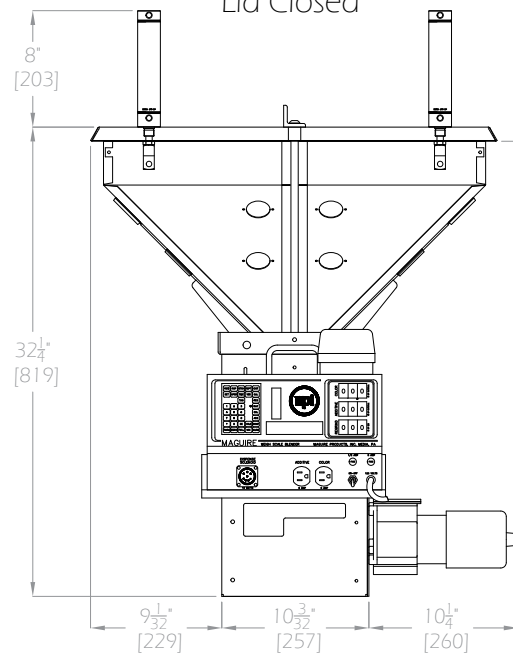
WSB-140MP SIDE VIEW Lid Closed
