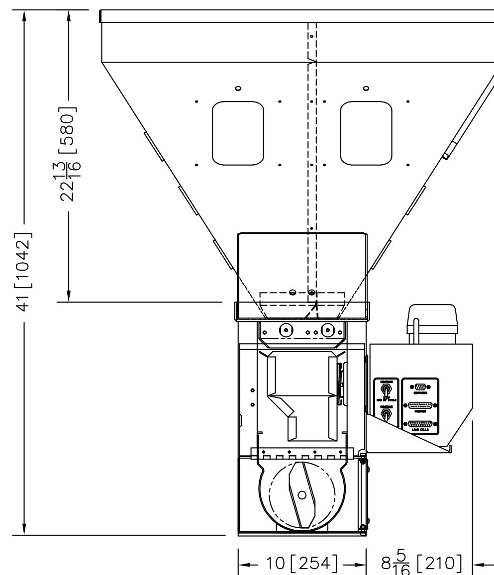
WSB 140 FRONT VIEW
