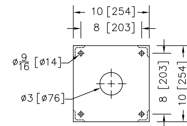
WSB 140 FOOTPRINT
