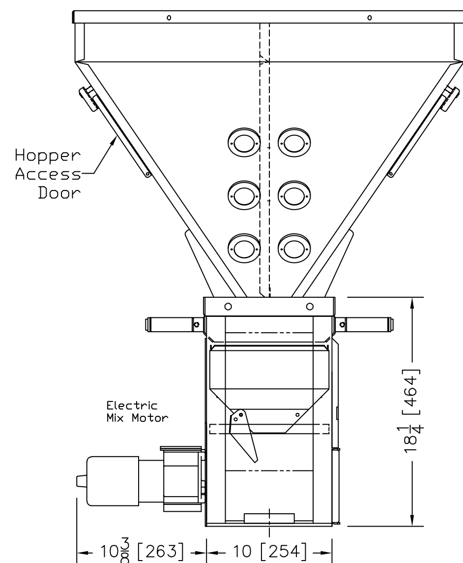
WSB 140 SIDE VIEW
