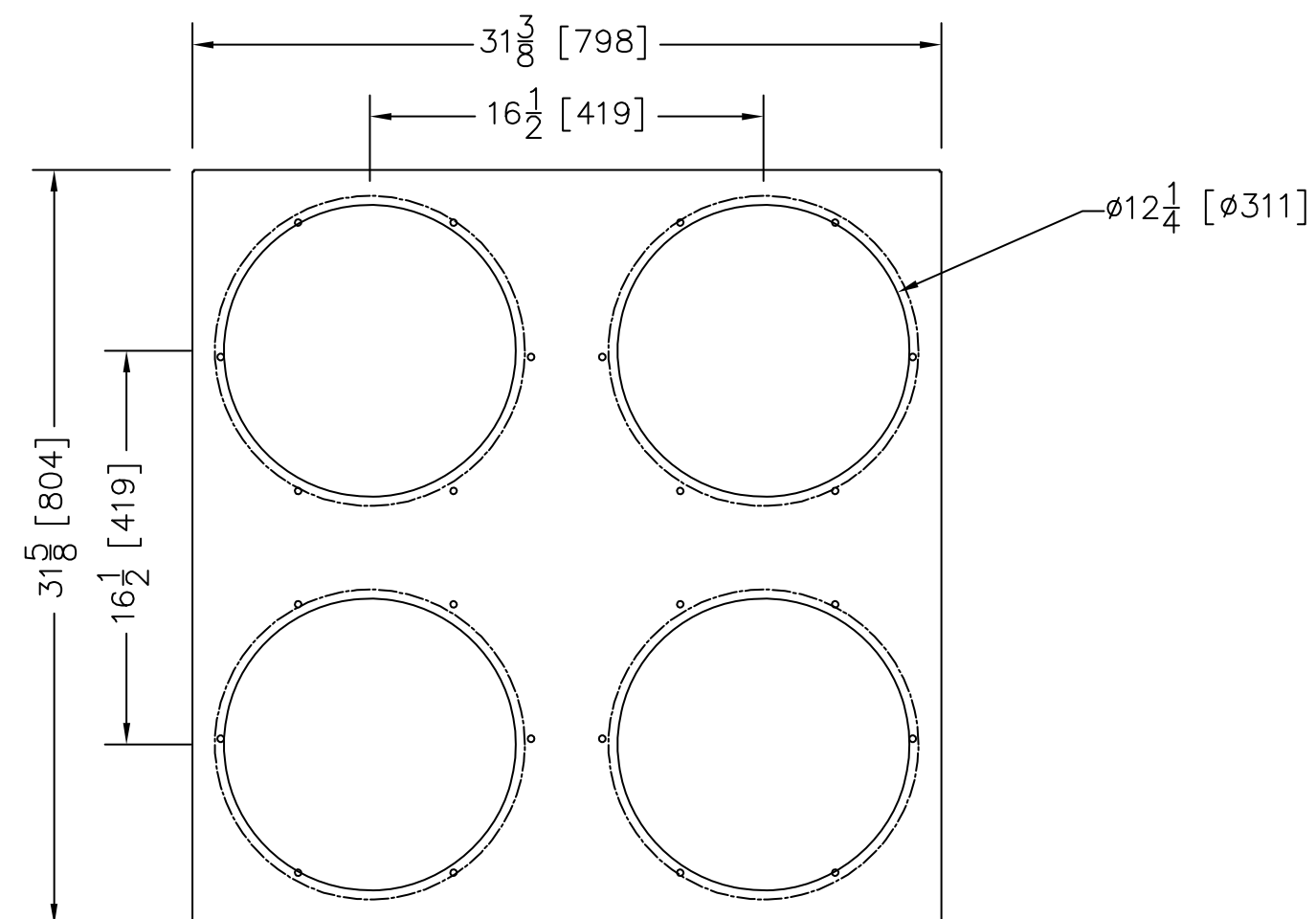
WSB 140 LID TOP VIEW
