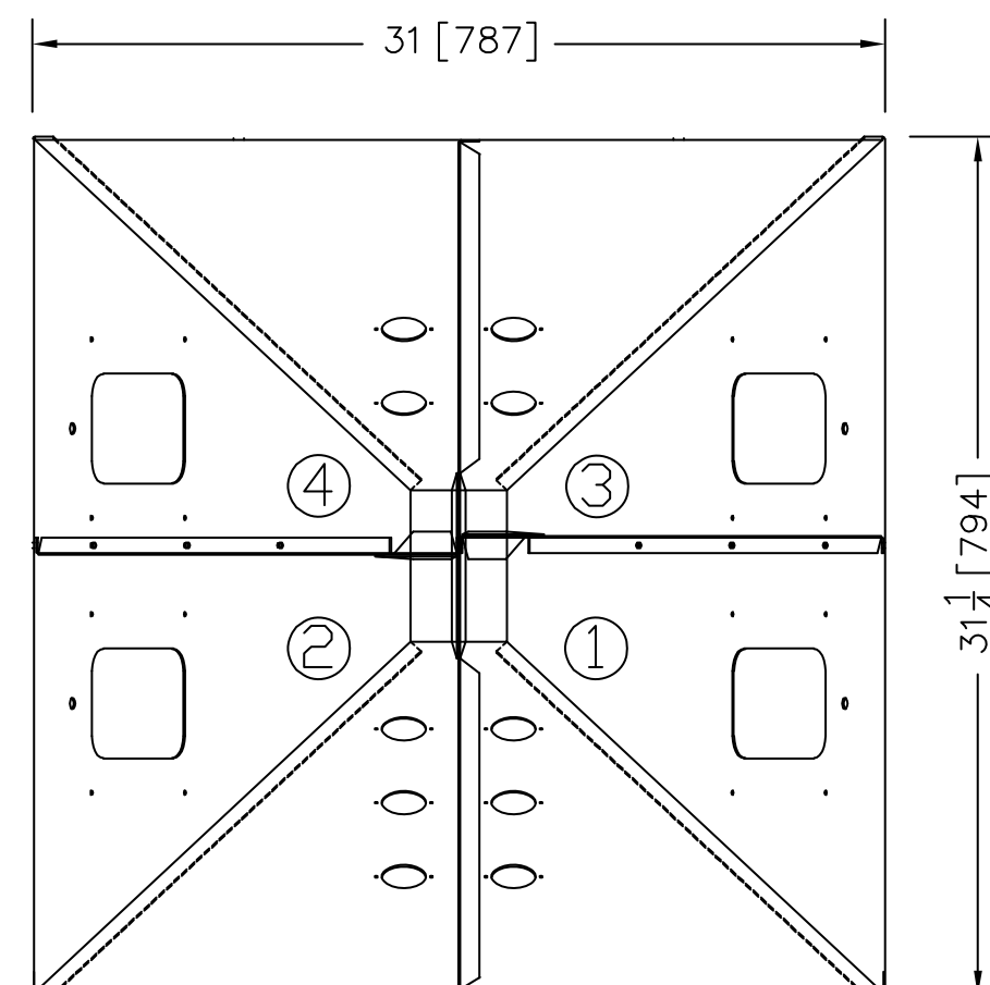
WSB 140 HOPPER TOP VIEW Controller Side
